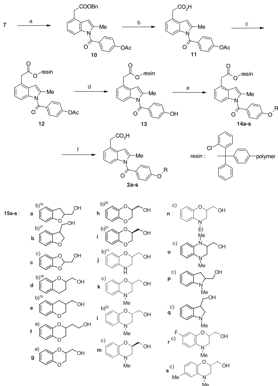
Scheme 2. Synthesis of 2a–s . Reagents: (a) NaOH (powdered), p -acetoxybenzoyl chloride, \text{CH}_2\text{Cl}_2 ; (b) \text{Pd}(\text{OH})_2 , \text{H}_2 , \text{EtOAc} ; (c) resin, diisopropylethylamine; (d) piperidine, \text{CH}_2\text{Cl}_2 ; (e) 15a–s , DEAD, \text{PPh}_3 ; (f) \text{AcOH} , \text{CF}_3\text{CH}_2\text{OH} , \text{CH}_2\text{Cl}_2 . (a) Commercially available; (b) reported; (c) described in Scheme 3a–h.
