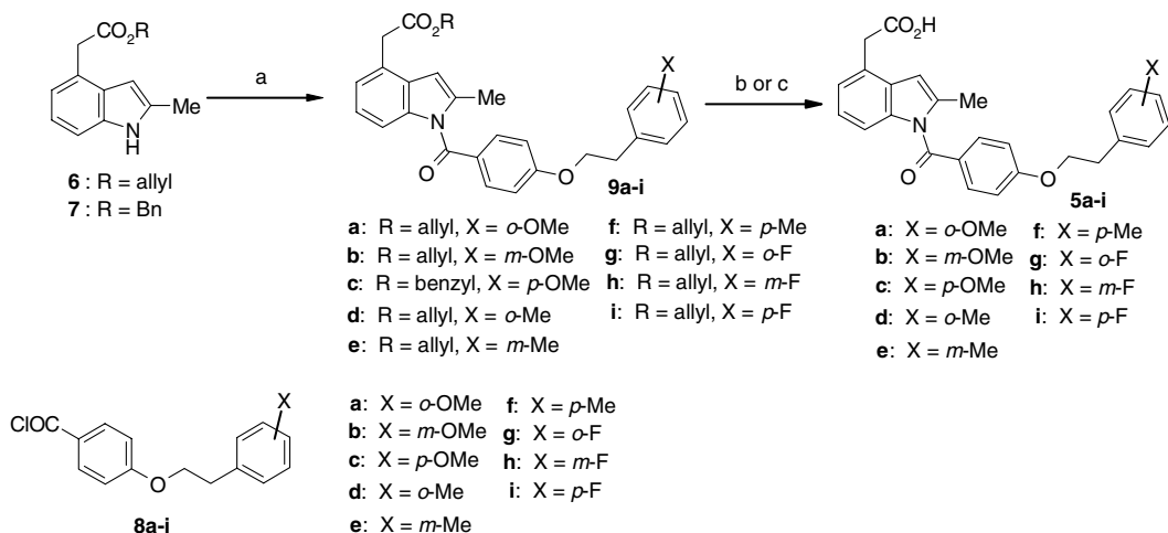
Scheme 1. Synthesis of 5a-i. Reagents: (a) NaOH (powdered), 8a-i, TBACl, H 2 Cl 2 ; (b) morpholine, Pd(PPh 3 ) 4 , THF; (c) H 2 , Pd-C, MeOH, EtOAc.
