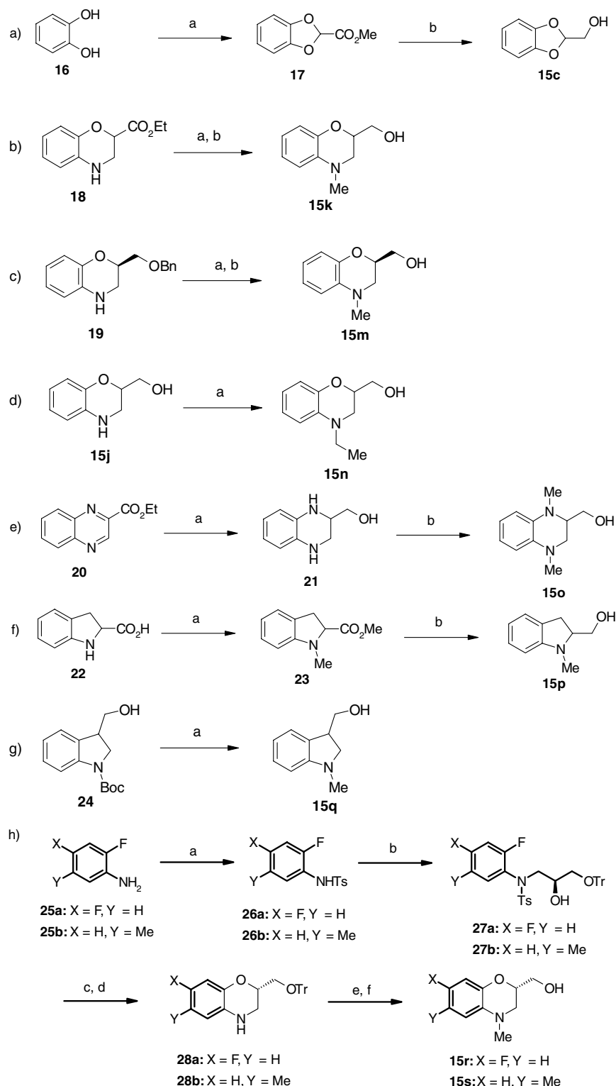
Scheme 3. Synthesis of 15c , 15k , and 15m–s . (a) Reagents: (a) NaH, methyl dichloroacetate, DMF; (b) LiAlH 4 , THF. (b) Reagents: (a) K 2 CO 3 , MeI, acetone; (b) LiAlH 4 , THF. (c) Reagents: (a) K 2 CO 3 , MeI, acetone; (b) H 2 , Pd–C, HCl, MeOH. (d) Reagents: (a) K 2 CO 3 , EtI, DMF. (e) Reagents: (a) NaBH 4 , MeOH, THF; (b) K 2 CO 3 , MeI, acetone. (f) Reagents: (a) K 2 CO 3 , MeI, acetone; (b) LiAlH 4 , THF. (g) Reagents: (a) LiAlH 4 , ether. (h) Reagents: (a) TsCl, Pyridine, CH 2 Cl 2 ; (b) (S)-(-)-glycidyl triphenylmethyl ether, K 2 CO 3 , BnEt 3 NCl, 1,4-dioxane; (c) t BuOK, THF; (d) Na, naphthalene, DME; (e) MeI, K 2 CO 3 , acetone; (f) AcOH, THF, H 2 O.
